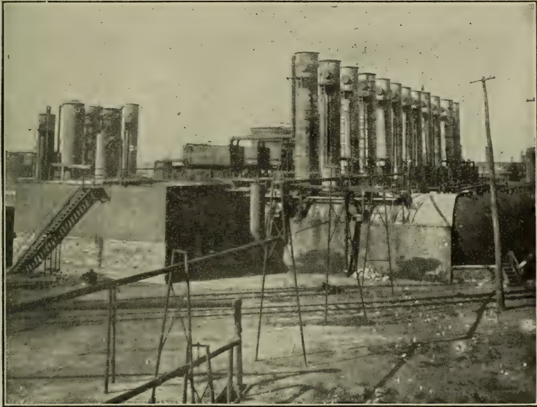
From "The American Petroleum Industry," by Bacon and Hamor. FIG. 107.—Tower System for Distilling Petroleum.
